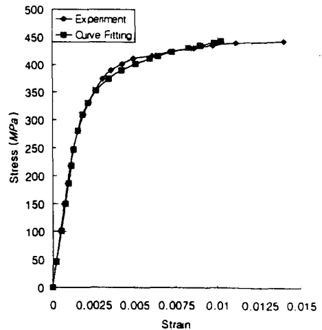
Fig. 4 Comparison of stress-strain curves obtained by experiments and curve fittings
