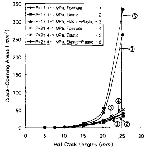
Fig. 6 Axial crack-opening areas ( r_m=7.1 mm, t=1.7 mm)
