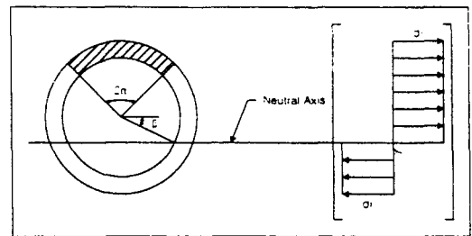
Fig. 1 Fully plastic stress distribution
